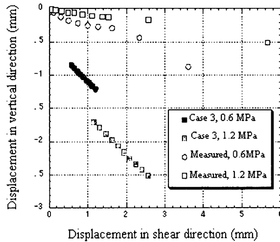
Fig. 7 Vertical vs. shear displacement of concrete block
